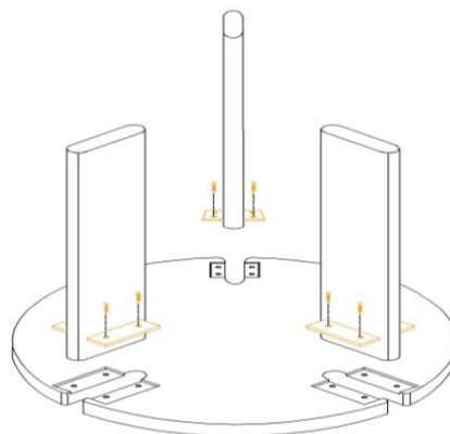
IMAGE 5 - ALL 3 BASE ASSEMBLY WITH TOP
